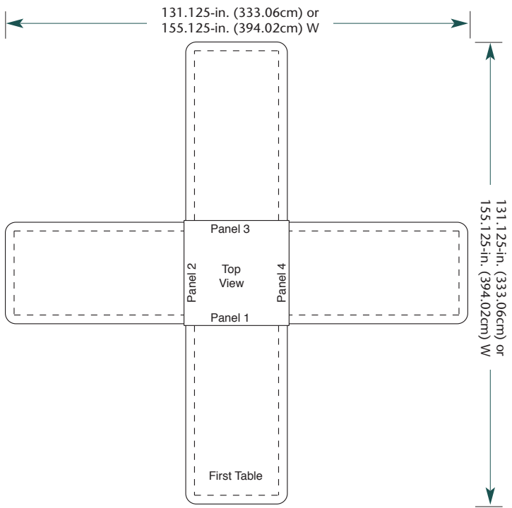
+, 4-Station
