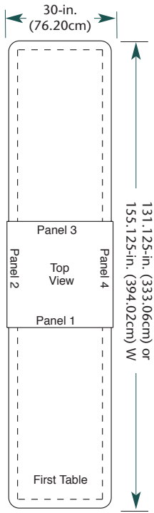
In-Line, 2-Station
