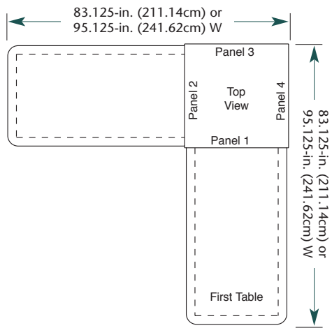
L, 2-Station
